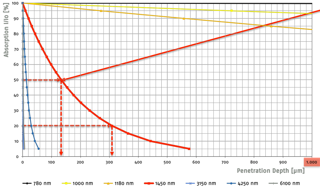
Penetration Depth and Absorption, radiation angle compensated
